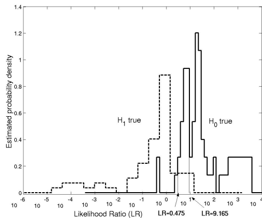
Figure 3: Estimated probability density functions of LRs.
